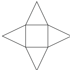
Pyramide
