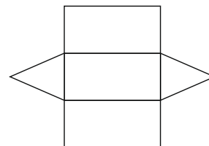
Prisma
