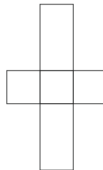
Quader
